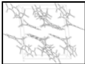
Fig. 2. Packing diagram of the title compound viewed down the b axis, showing the chains of molecules formed by intermolecular hydrogen bonds (dashed lines).
